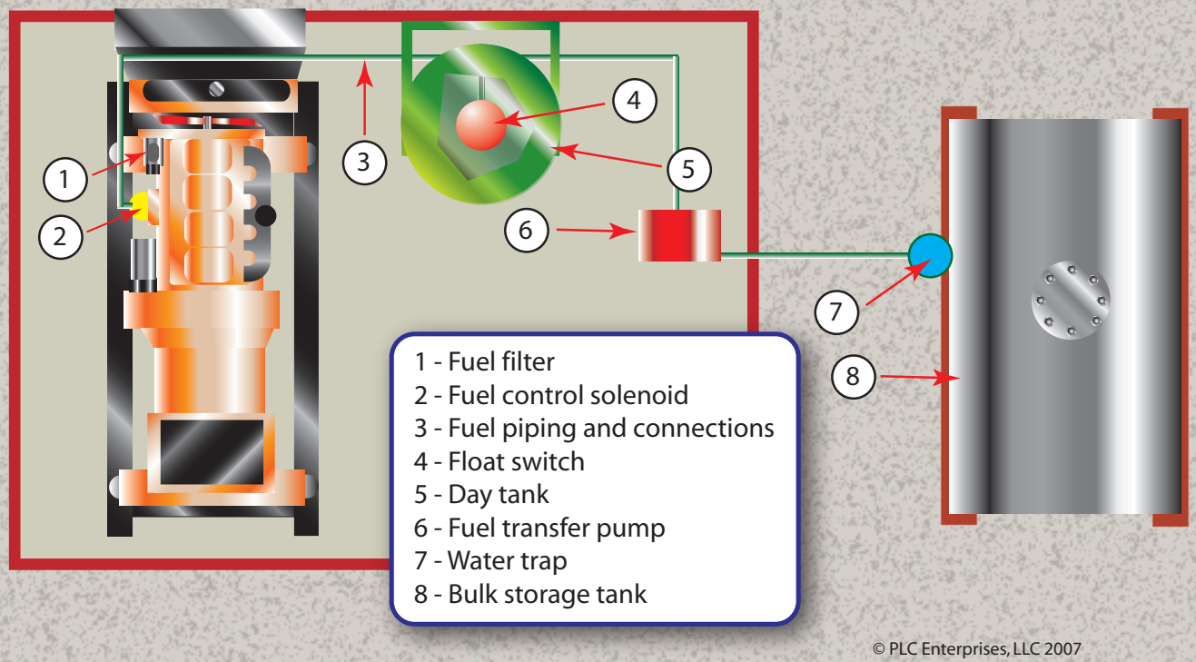
Diagram - Fuel System Maintenance Points
